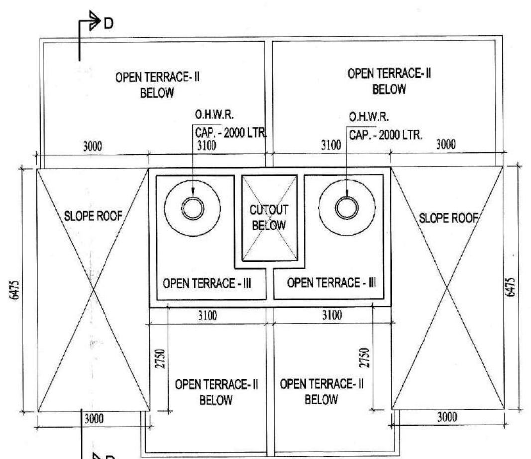
ROOF PLAN
